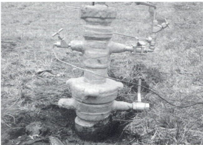
#2A Wax-Tape (aluminum pigmented) easily applied to a difficult-to-protect wellhead. Note the complete conformity to the irregular surfaces.
